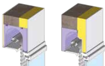
Coffre tunnel 1/2 linteau
