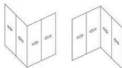
Galandage angle (32 mm)
